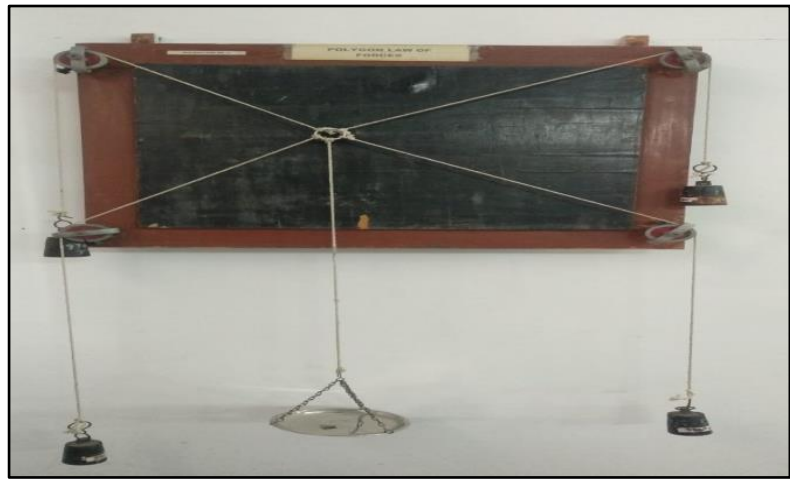
Polygon law apparatus
